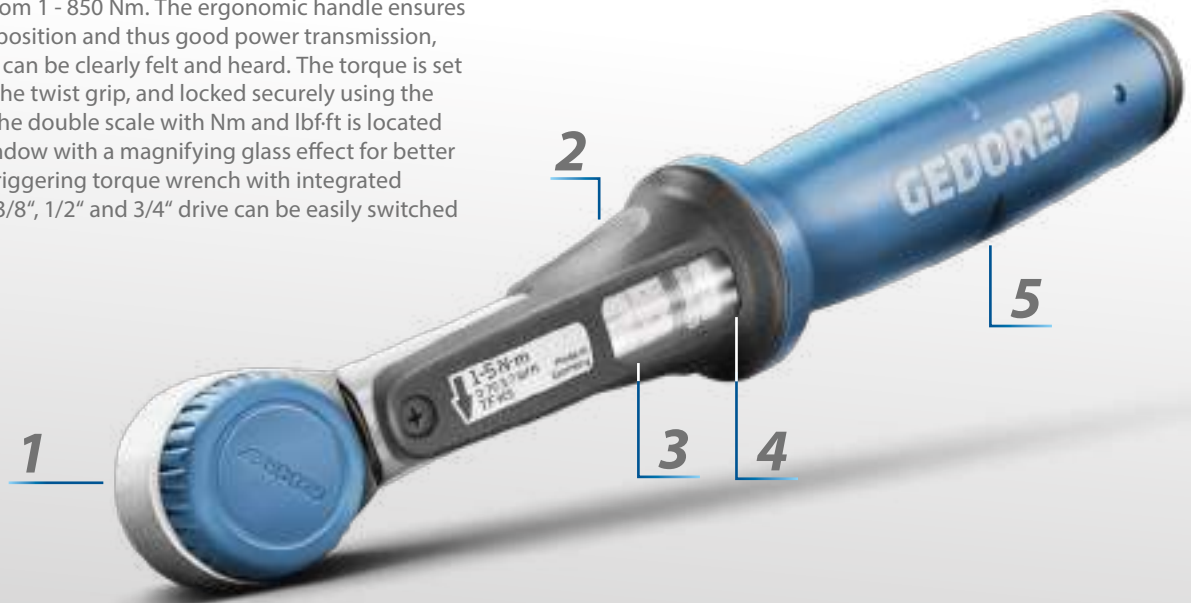
Torque wrench TORCOFIX TF-K 1/4"-3/4" 1-850 Nm TF-K
