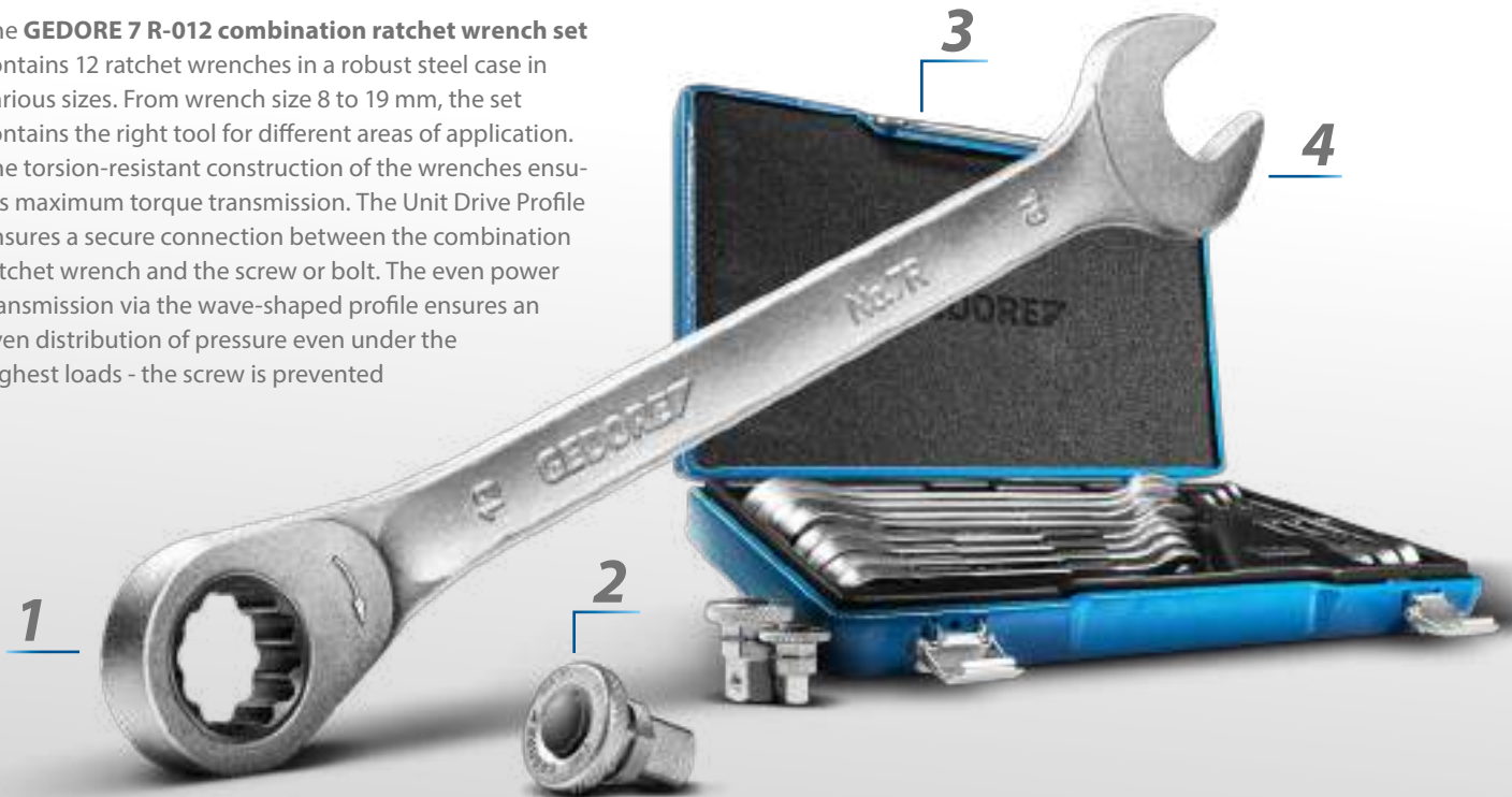
Set of open-end spanners with ring ratchet 7 R-012
